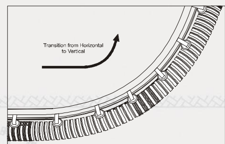
Fig 2. ICS Belt transition from horizontal to incline
