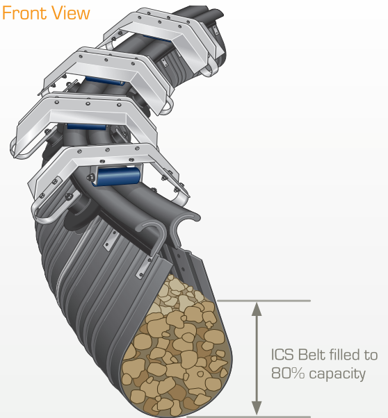
ICS Belt Transition from Horizontal to Incline Curve
